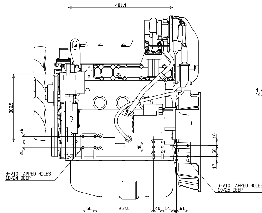
Starter side
