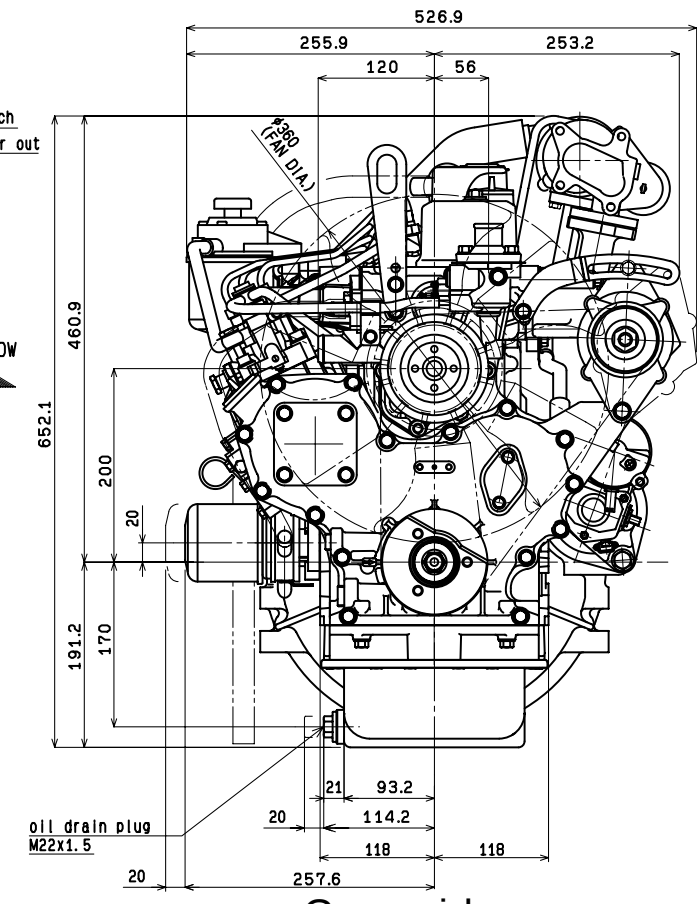
Gear side
