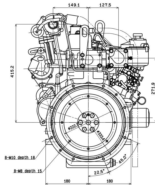
Flywheel side
