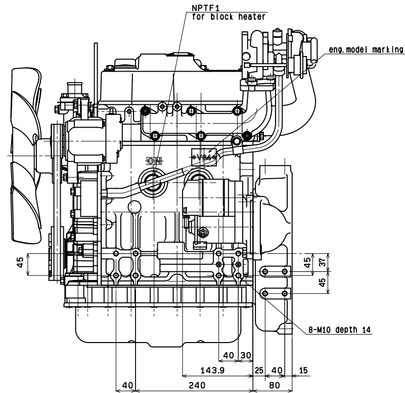
Starter side
