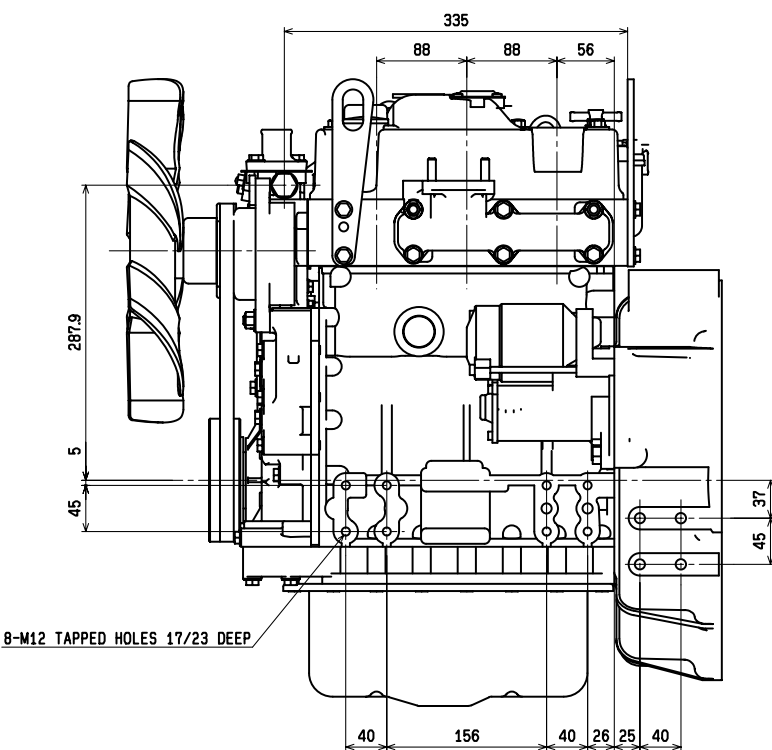
Starter side
