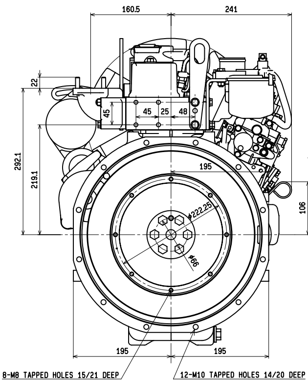
Flywheel side
