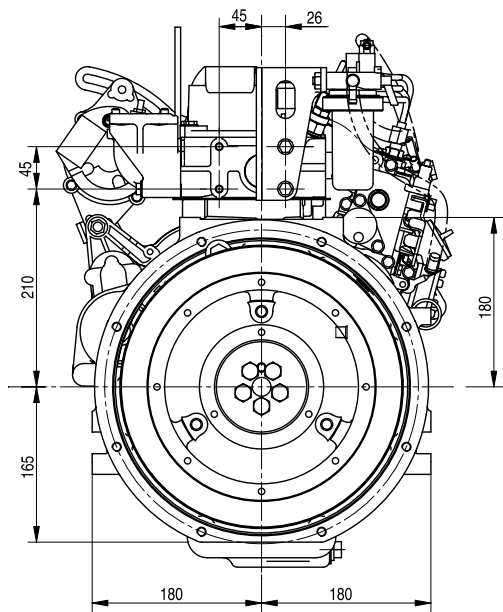
Flywheel side
