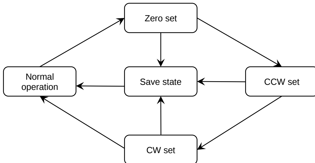
Figure 1 Azimuth indicator calibration state chart
