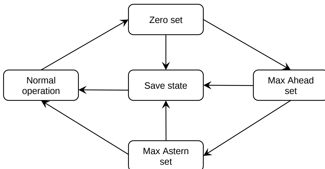
Figure 2 General indicator calibration state chart
