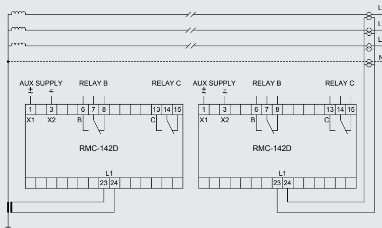
Protection of the voltage source and the load network
