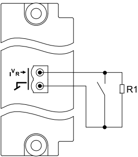
Figure 4.23 Connection of a dry contact with cable supervision
