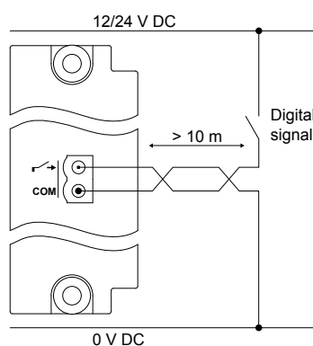
Figure 4.12 Example: Twisted wire for compliance with EN60255-26
