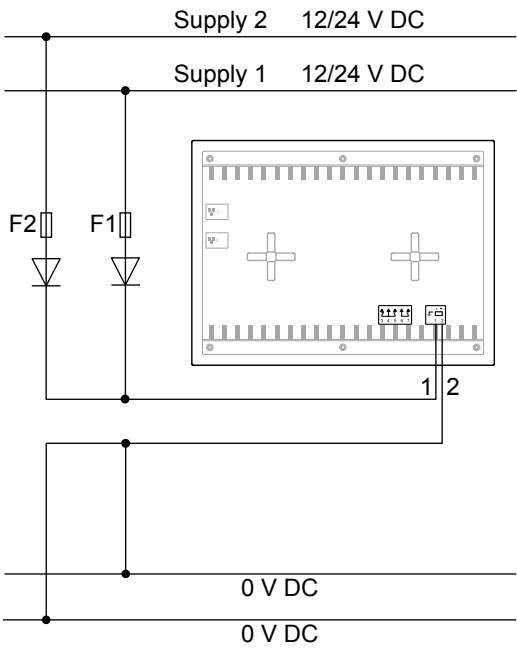
Figure 4.86 Example of a power supply and backup connected to the power supply terminals
