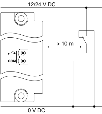
Figure 4.22 Example: Closed contact for compliance with EN60255-26
