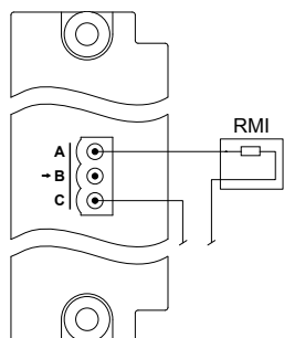
Figure 4.39 Connection of a 1-wire resistance measurement input (RMI)
