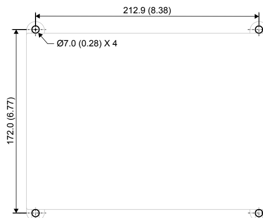
Drilling template *
